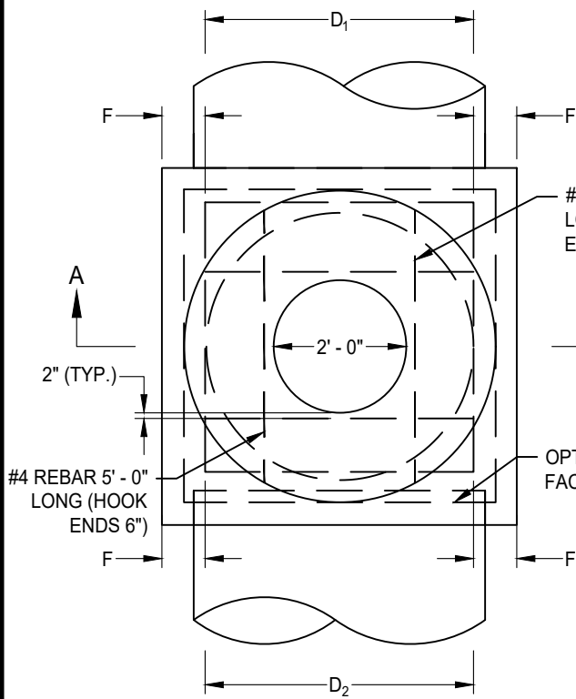
PLAN
