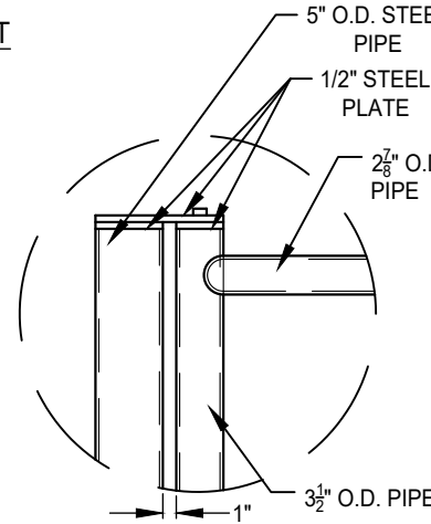
GATE TIE-DOWN POST
